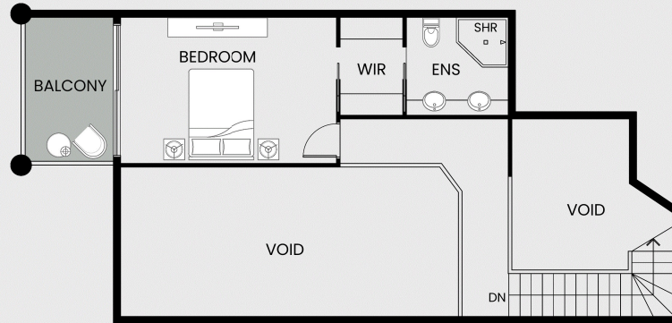
UPPER LEVEL PLAN
